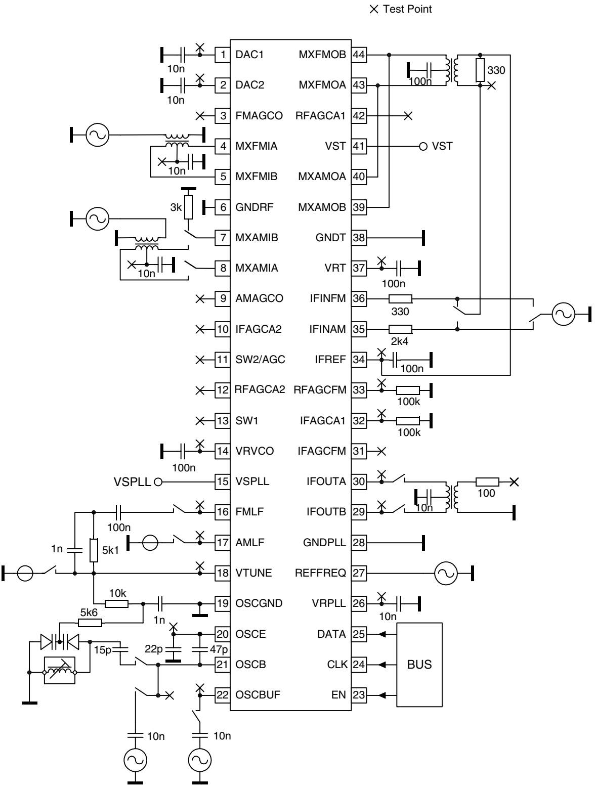
Figure 13. Test Circuit
