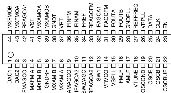
Figure 1. Pinning SSO44
