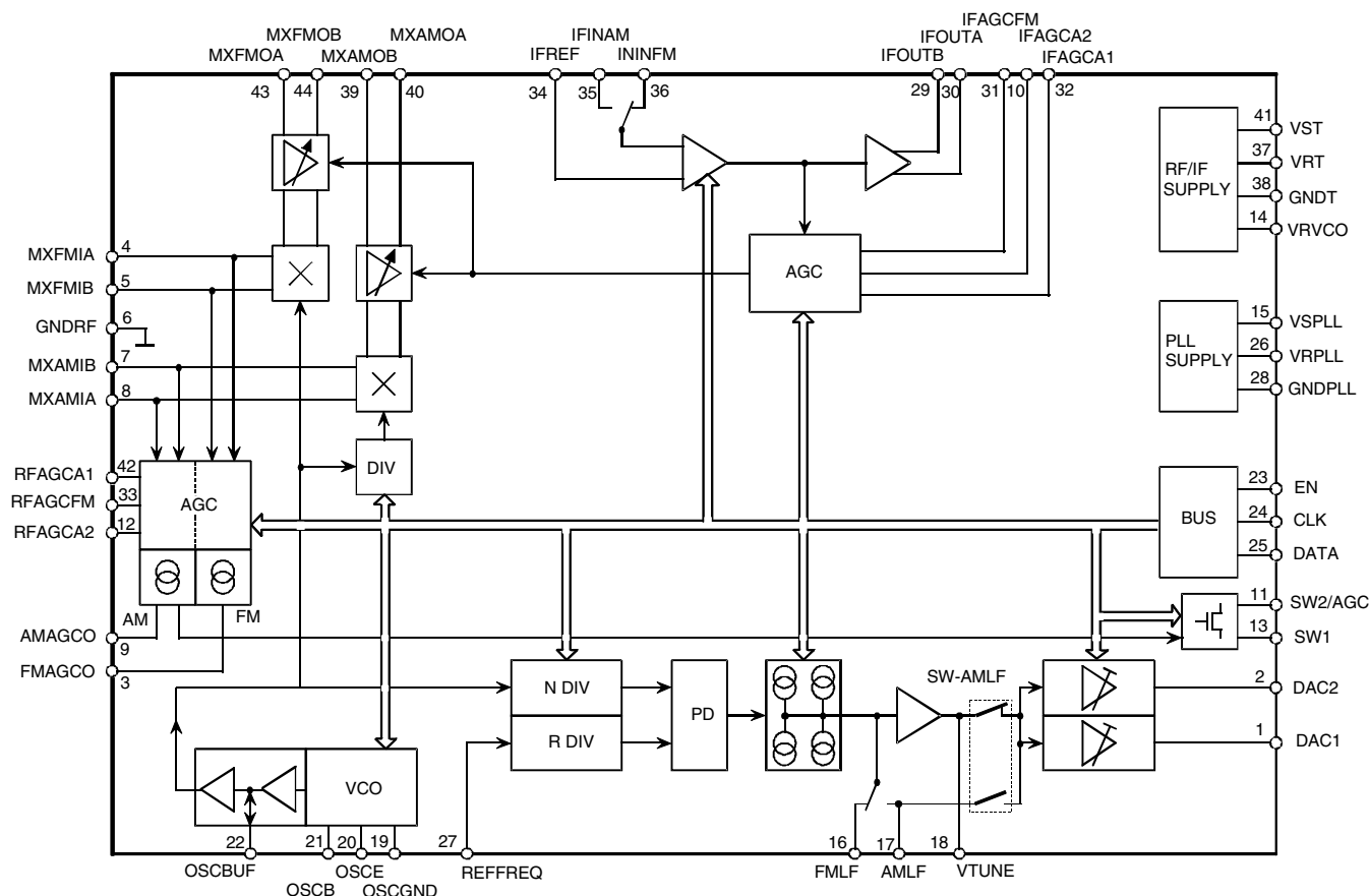
Figure 2. Block Diagram
